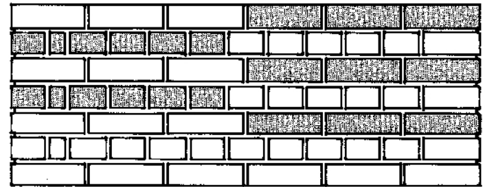
English Bond English Corner Dutch Corner
