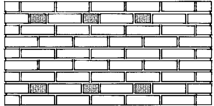
Common Bond Flemish Headers Every 6th Course
