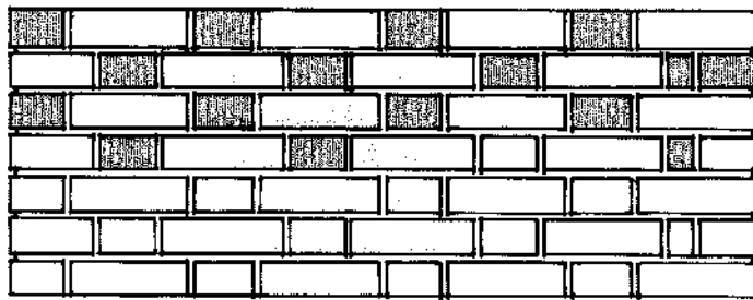
Flemish Bond Dutch Corner English Corner
