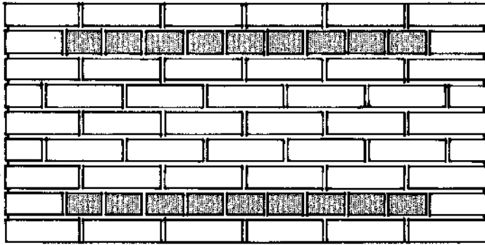
Common Bond Full Headers Every 6th Course
