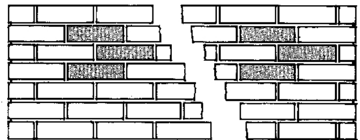
Running Bond 1/2 Bond 1/3 Bond
